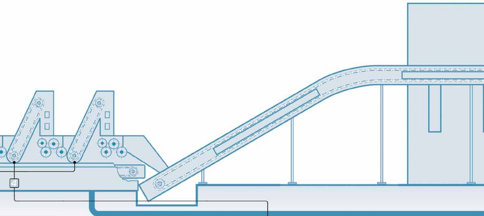
3 ESTEIRA DE CANA MAIN CANE CARRIER CONDUCTOR DE CAÑA
